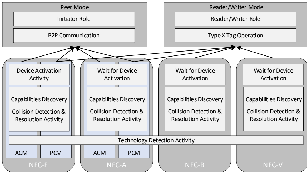
Figure 11: Polling Architecture
