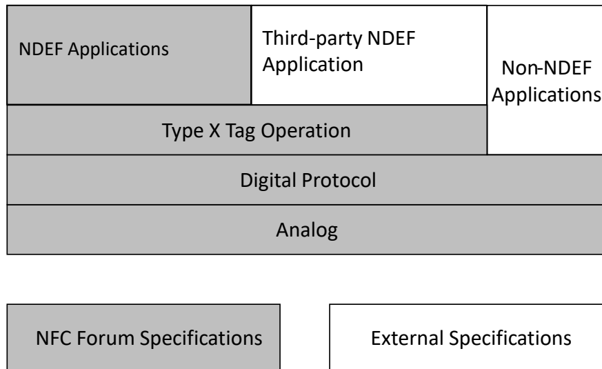
Figure 9: Reader/Writer Mode Architecture
