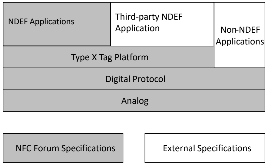
Figure 10: Tag Mode Architecture
