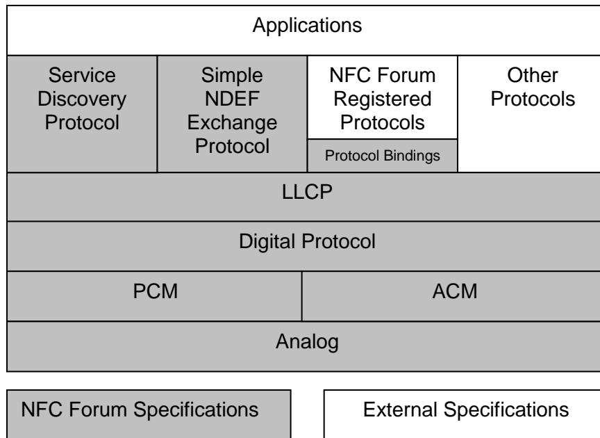
Figure 8: Peer Mode Architecture
