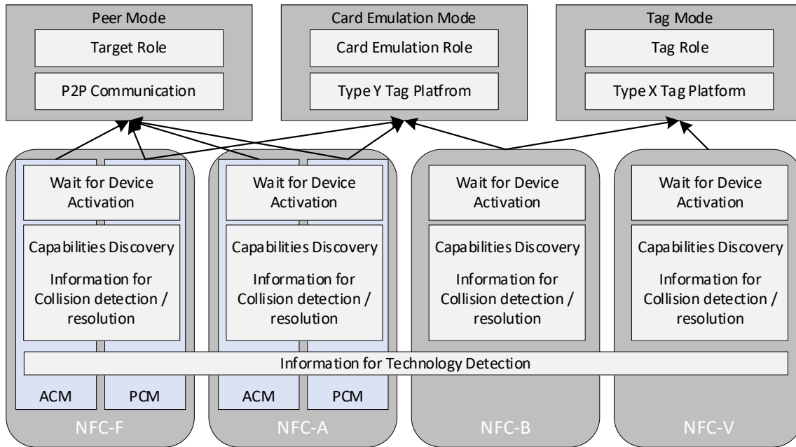
Figure 12: Generic Listening Architecture
